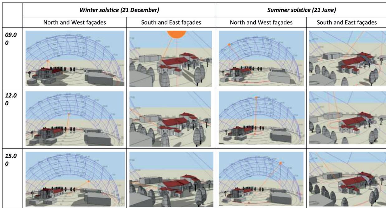
Fig. 19. Shading analysis in the Cypriot pilot building.
