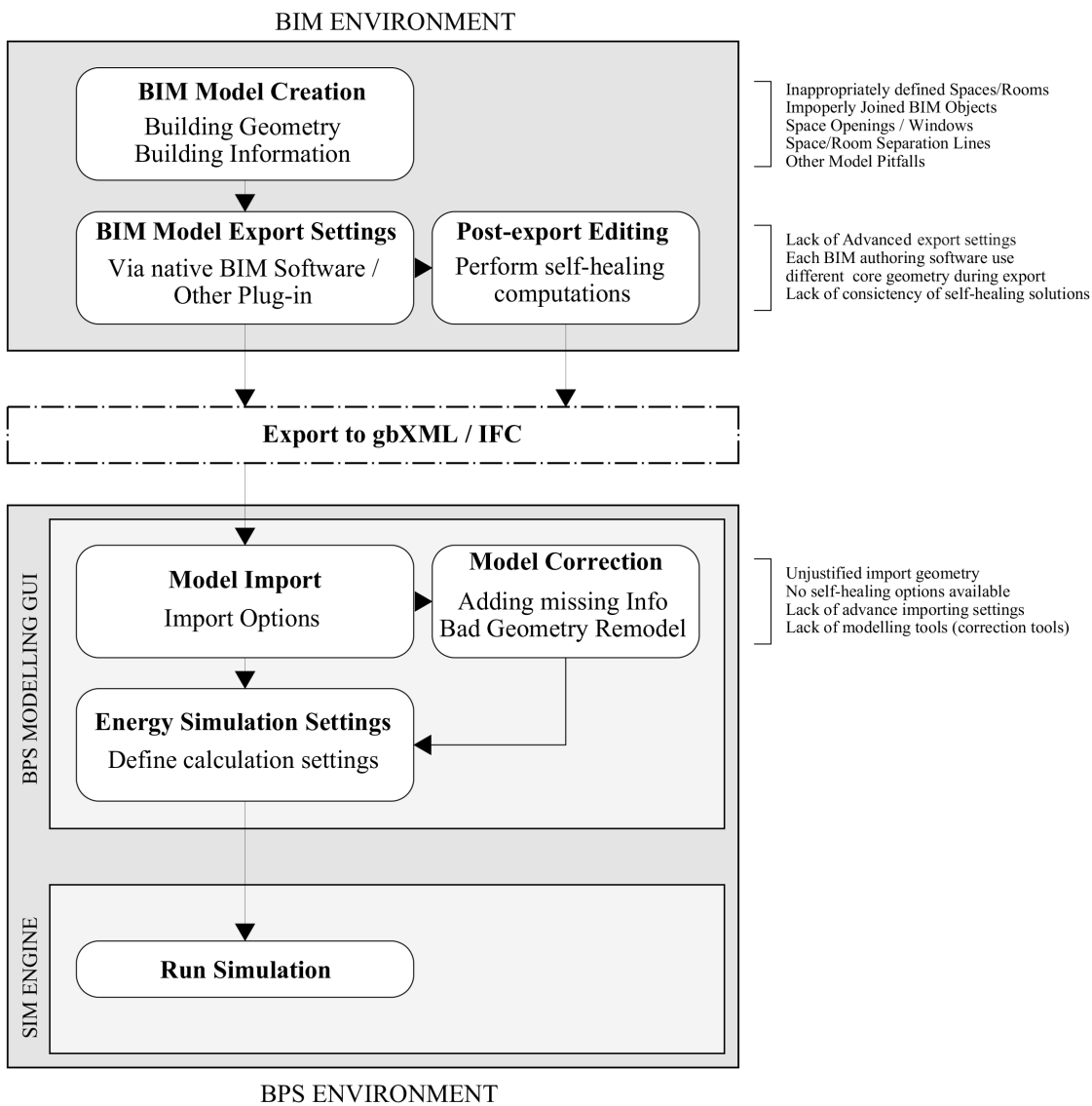
Fig. 26. Schematic representation of BIM to BPS Interoperability problem
