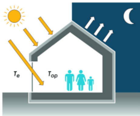
Fig. 34. Idealised thermal diurnal performance of extremely lightweight (top) and high mass (bottom) building. T_e and T_{op} correspond to outdoor and indoor temperature respectively. Source: Košir 2019.
