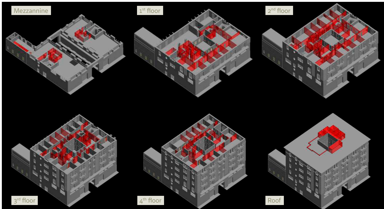
Fig. 22. Post-operam EE-HBIM model of the Egyptian case study – Cordahi Building.
