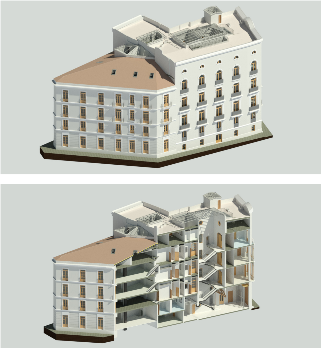
Fig. 9. Render view of the EE- HBIM model of the Spanish pilot building “Palacio de Calatayud” in Valencia.
