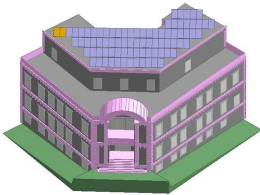
Fig. 14. Energy model of the Municipality of Tripoli showing the PV and SWH panels
