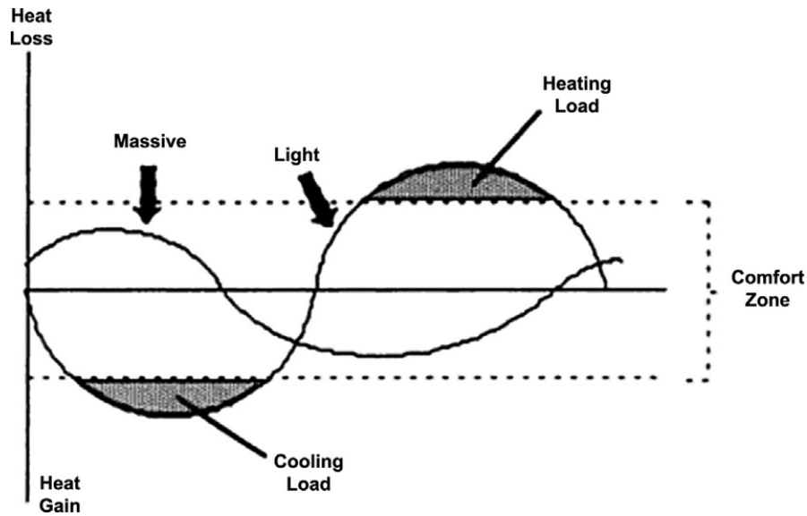
Fig. 33. Daily Building heating and cooling loads for buildings of massive and light construction. Source: Asimakopoulos, 1996.
