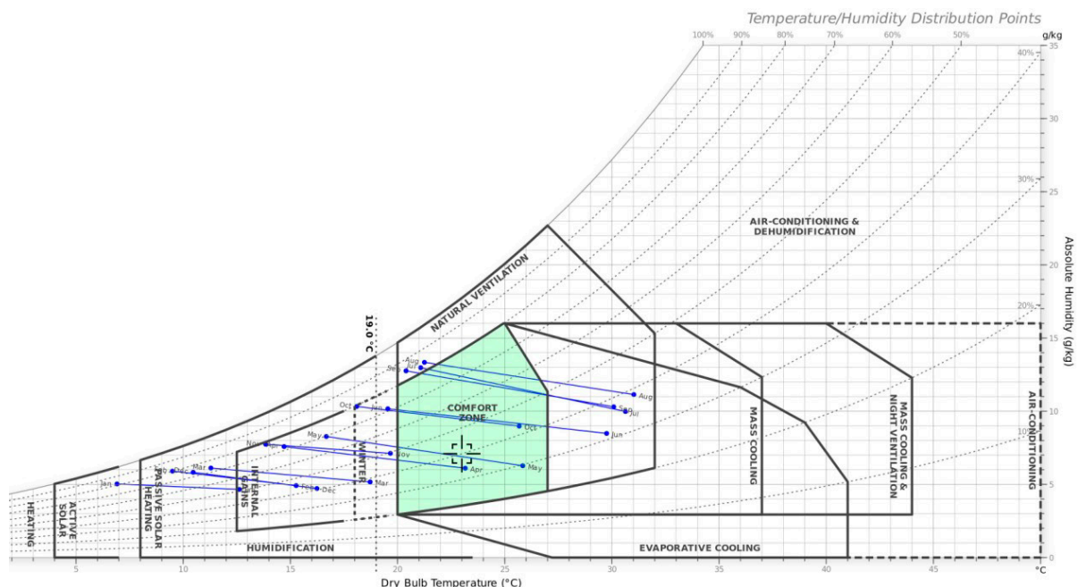
Fig. 20. Givoni comfort diagram for Bethlehem. Source: https://drajmarsh.bitbucket.io/psychro-chart2d.html
