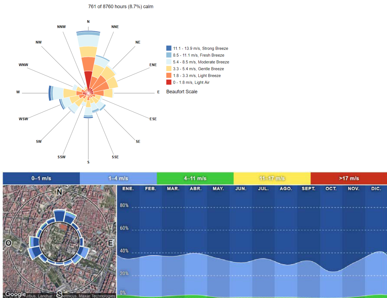
Fig. 17. The distribution and windspeed in València, colour coded into bands. The percentage of time spent at various speed ranges. Source: https://www.windfinder.com/windstatistics/valencia
