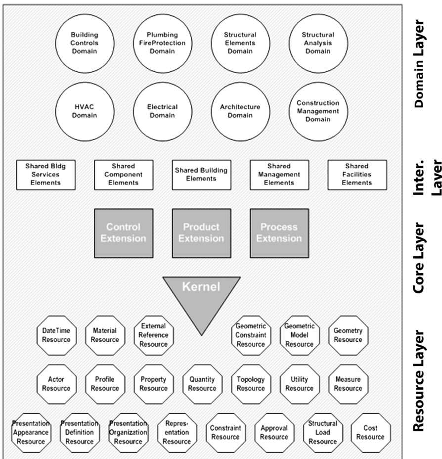
Fig. 29. IFC Data schema with four conceptual layers (buidingSMART 2020).
