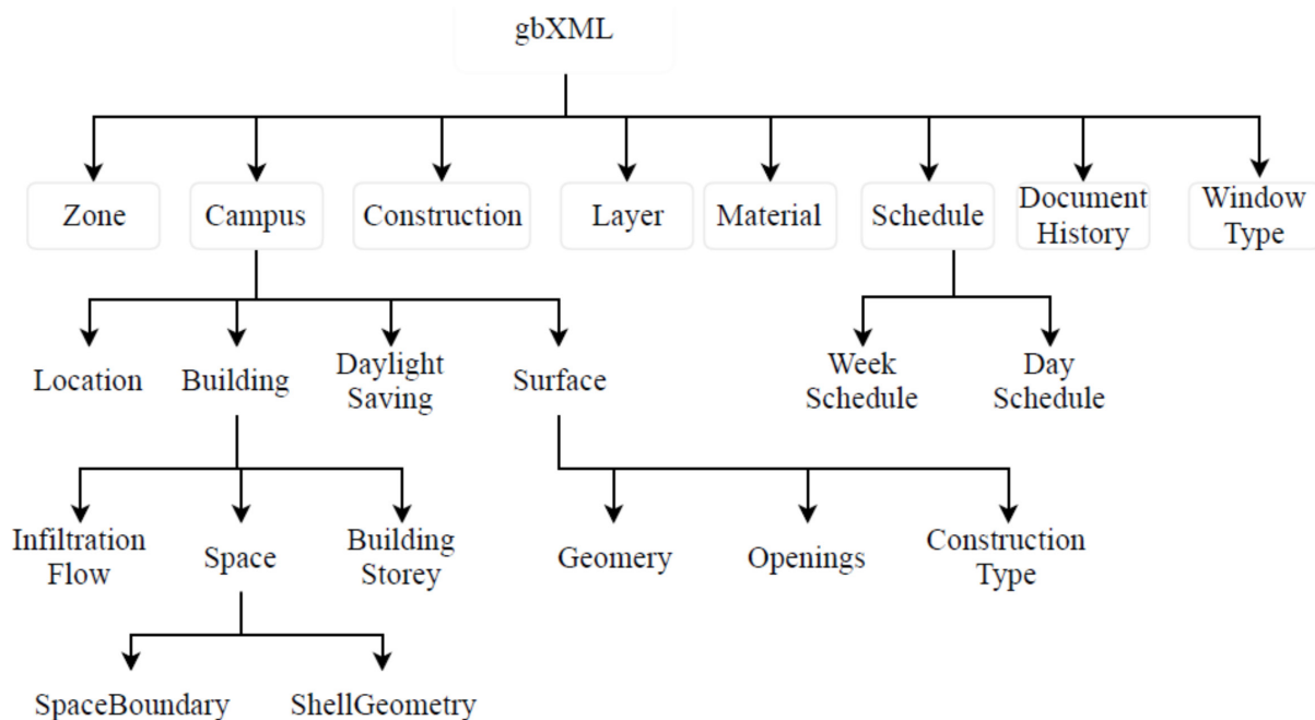
Fig. 30. Simplified hierarchy of information organisation in gbXML schema (Ham and Golparvar-Fard 2015).
