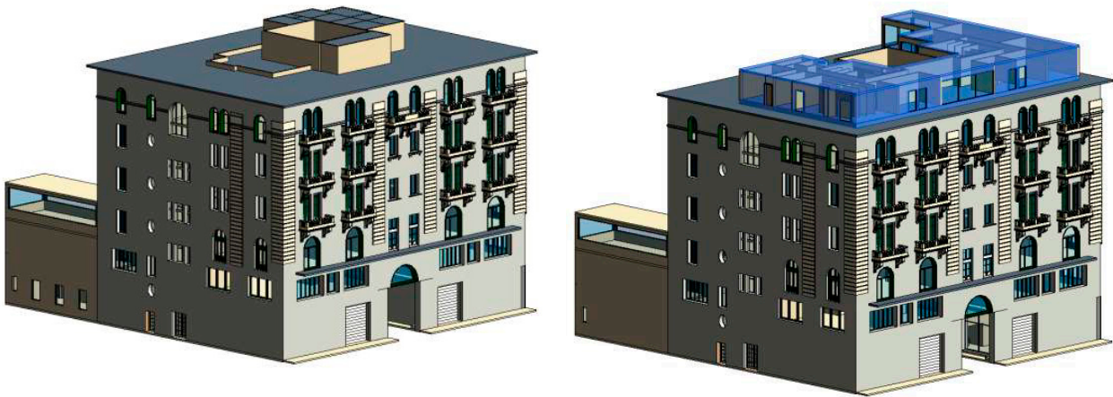
Fig. 23. Post-operam EE-HBIM model of the Egyptian case study – Cordahi Building.
