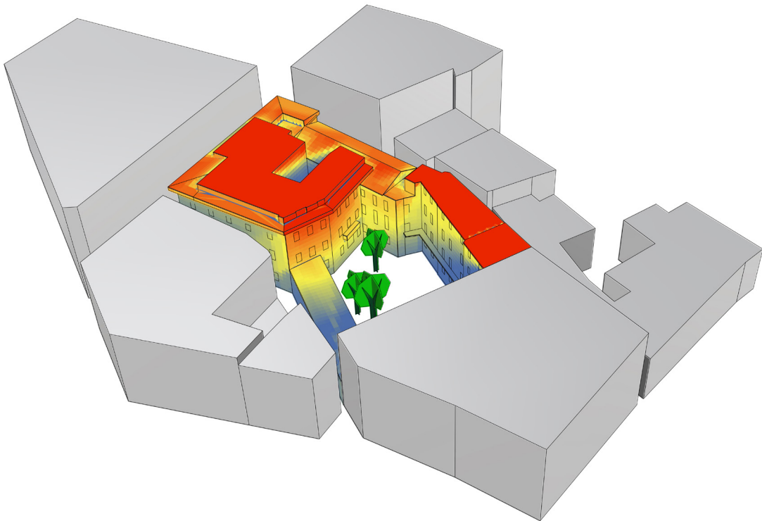
Fig. 5. Analysis of the sunshine duration on the façades of the Italian case study, to select the areas of minimum sunshine radiation to perform the Heat Flux meter analysis.
