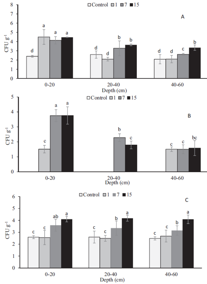
Fig. 4. Soil pathogen microbial biomass ( Salmonella/Shigella : A, Staphylococcus : B and Pseudomonas sp.: C) affected by the duration of wastewater application (0, 1, 7 and 15 years) at different soil depths 0–20, 20–40 and 40–60 cm. Different lower-case letters indicate significant differences among sampling sites and depths in according to Tukey post-hoc test ( p < 0.05 ).
